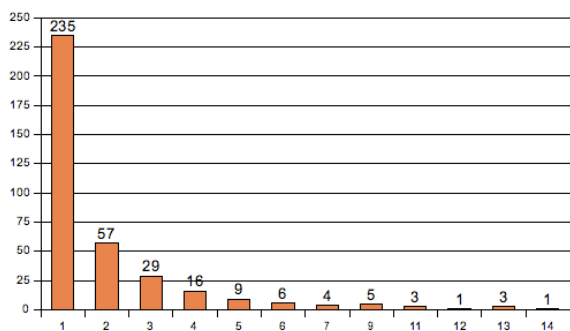
Figure 3. Distribution of 375 classes over the number of function names overloaded by a class.
