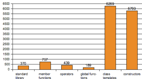
Figure 2. Distribution of 13817 overloaded function names over categories.
