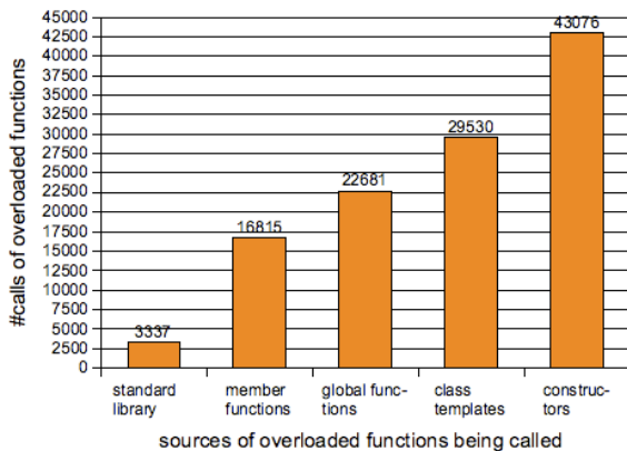
Figure 5. Distribution of 115439 calls of overloaded functions over categories.
