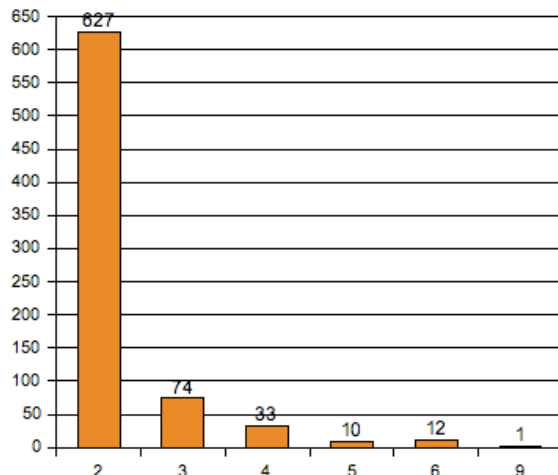
Figure 4. Distribution of 757 class members over the times they are overloaded.
